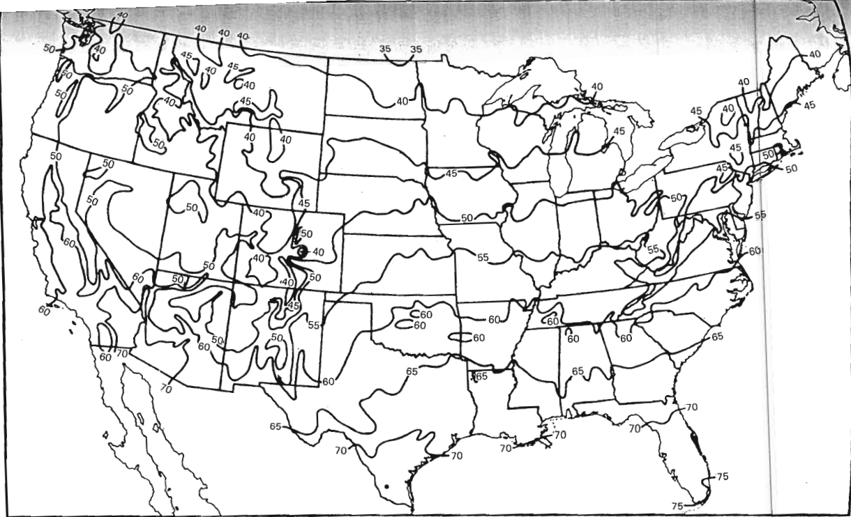
Fig. 26—Average annual temperatures in °F.
